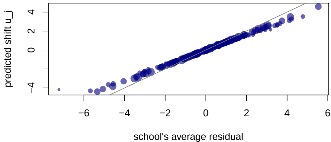
Figure 4: Predicted school shifts against the schools' average residuals. Every point lies between the 45-degree line and zero; small schools are pulled furthest.
